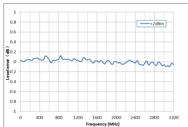
Measured level error versus frequency, Level = +2 dBm
