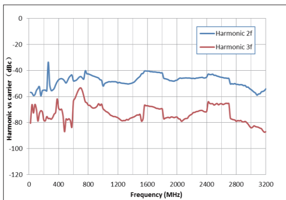
Measured harmonics versus carrier frequency at level ≤ +13 dBm
