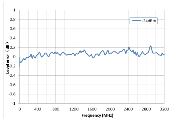
Measured level error versus frequency, Level = -24 dBm
